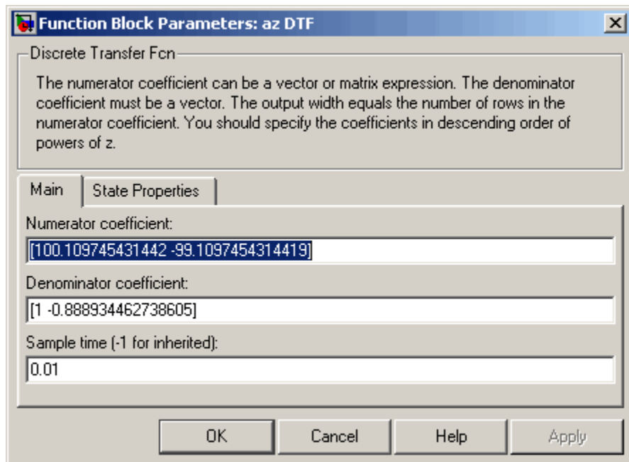
Mask of a Simulink compensator block
